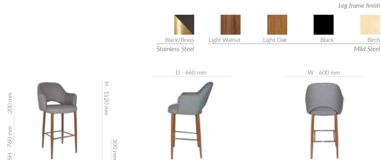
The model presented features Light Oak leg frames from solid ash, Gravity shell fabric, the Steel colour
