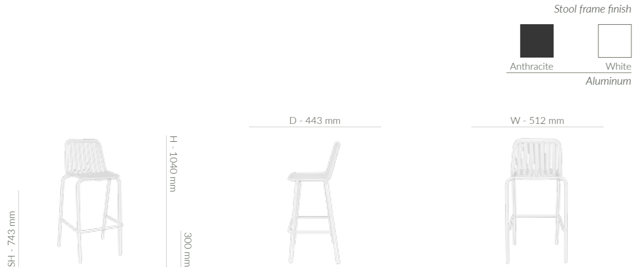
The model presented features the White finish, from aluminum
