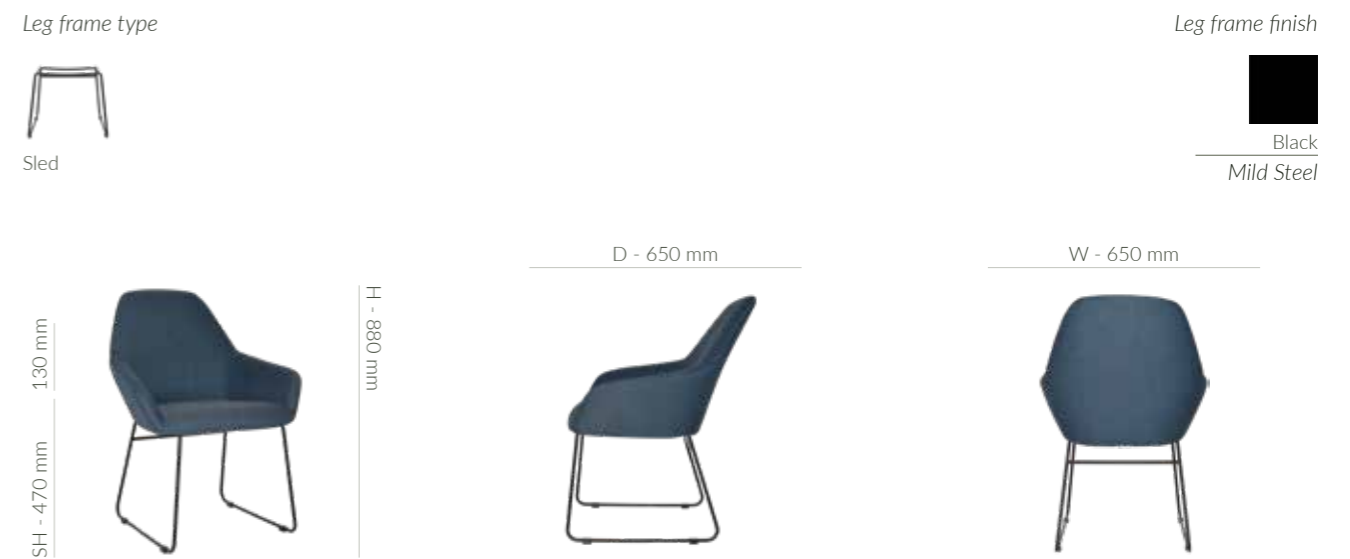
The model presented features Black Sled leg frames from mild steel, Gravity shell fabric, the Denim colour
