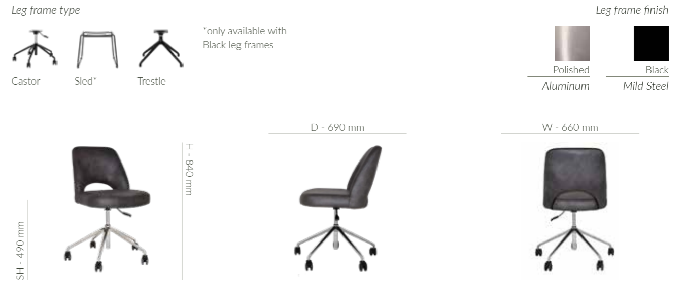
The model presented features Castor leg frames from polished aluminum, Eastwood shell fabric, the Slate colour
